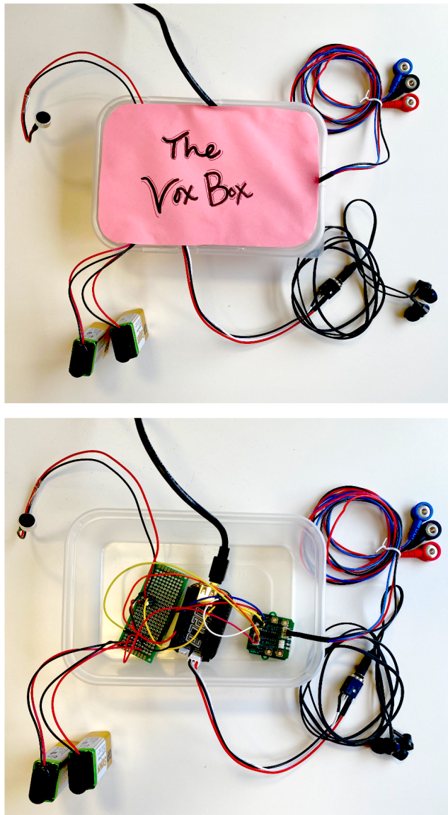
Figure 2: The VoxBox: external cables for electrodes, headphones, power supply (USB and 9 V batteries), and microphone (top), and inside a VoxEMG board, Bela Mini, and routing for power supply (bottom).
